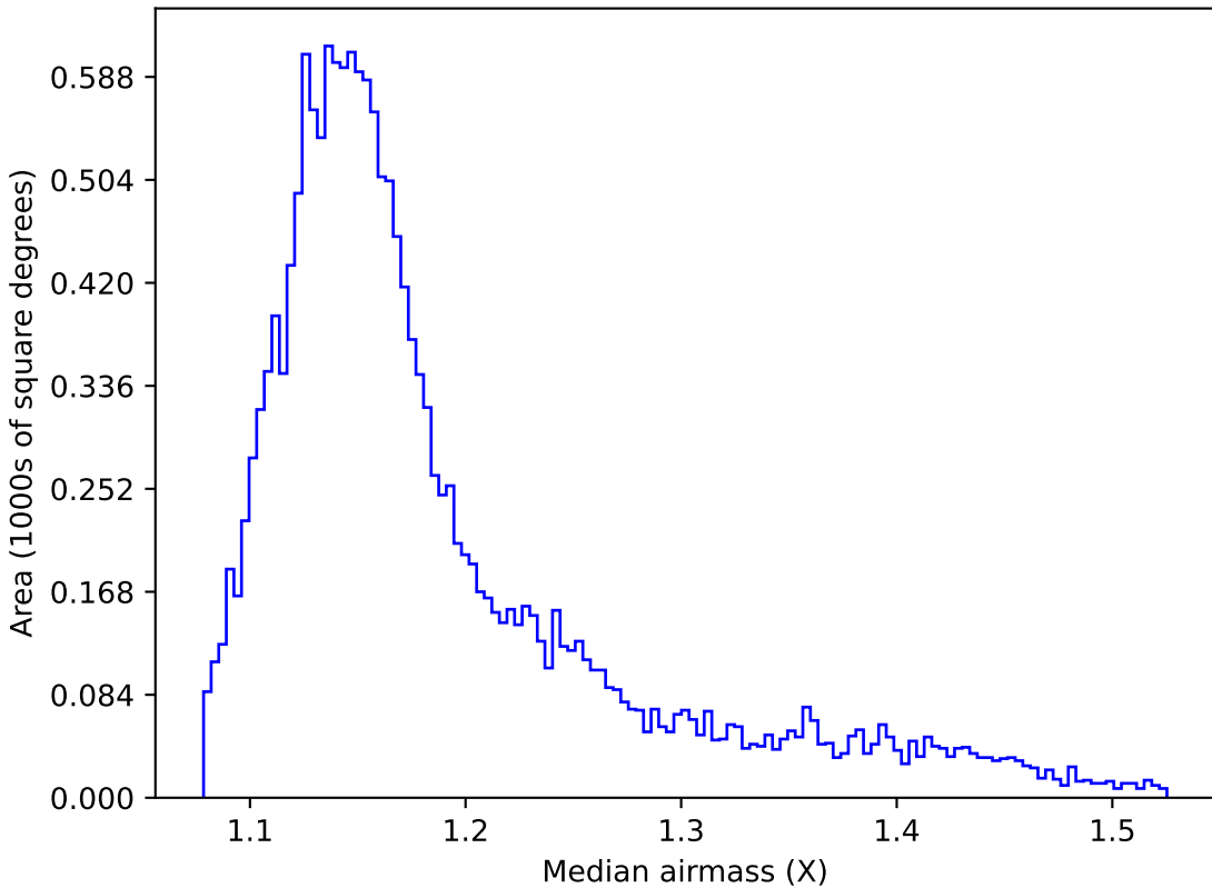
weather_cloudso8v3.4_10yrs WFD g band: Median airmass
