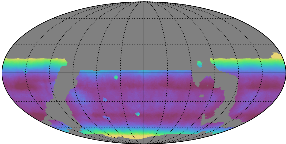
weather_cloudso8v3.4_10yrs WFD all bands: Median airmass
