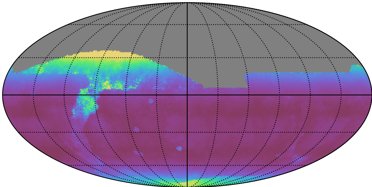
weather_cloudso8v3.4_10yrs All sky z band: Median airmass
