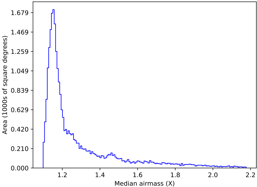
weather_cloudso8v3.4_10yrs All sky z band: Median airmass
