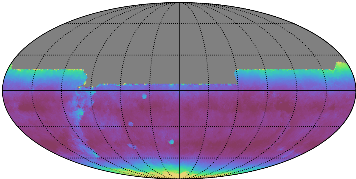
weather_cloudso8v3.4_10yrs All sky y band: Median airmass
