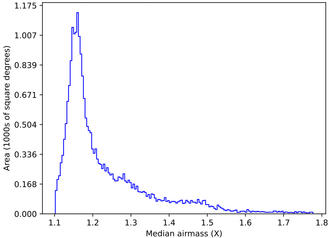
weather_cloudso8v3.4_10yrs All sky y band: Median airmass
