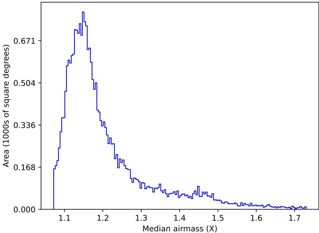
weather_cloudso8v3.4_10yrs All sky u band: Median airmass
