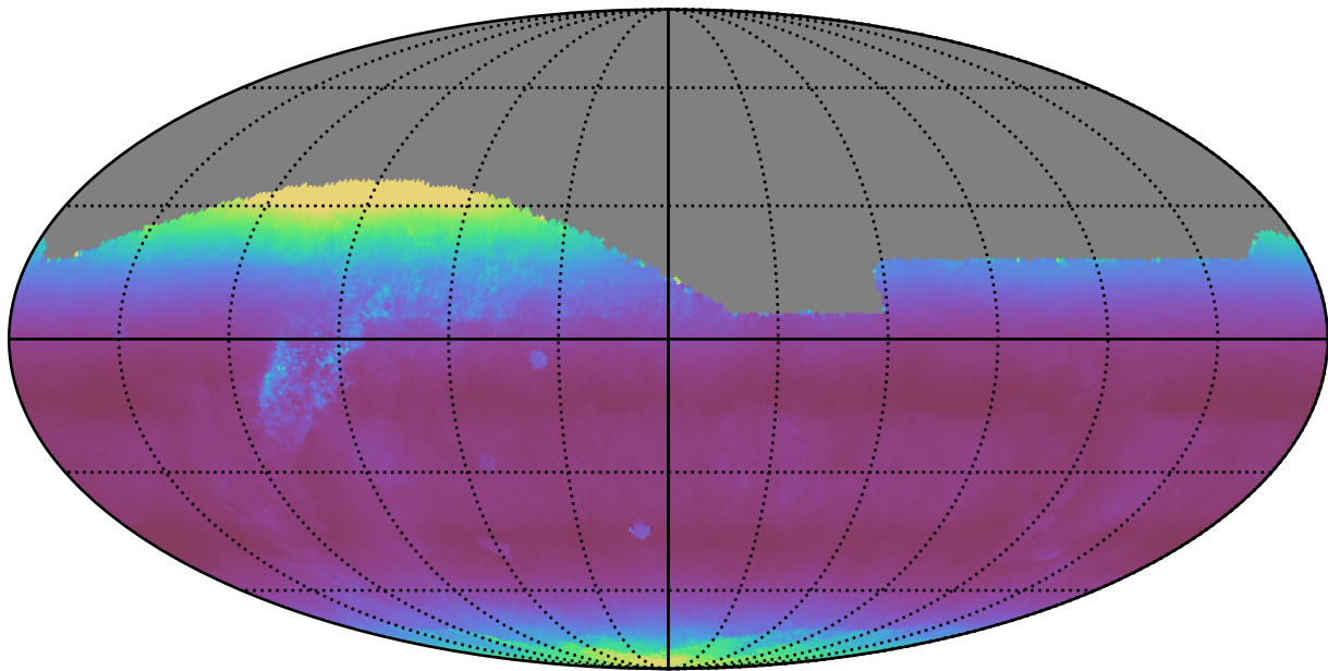
weather_cloudso8v3.4_10yrs All sky r band: Median airmass
