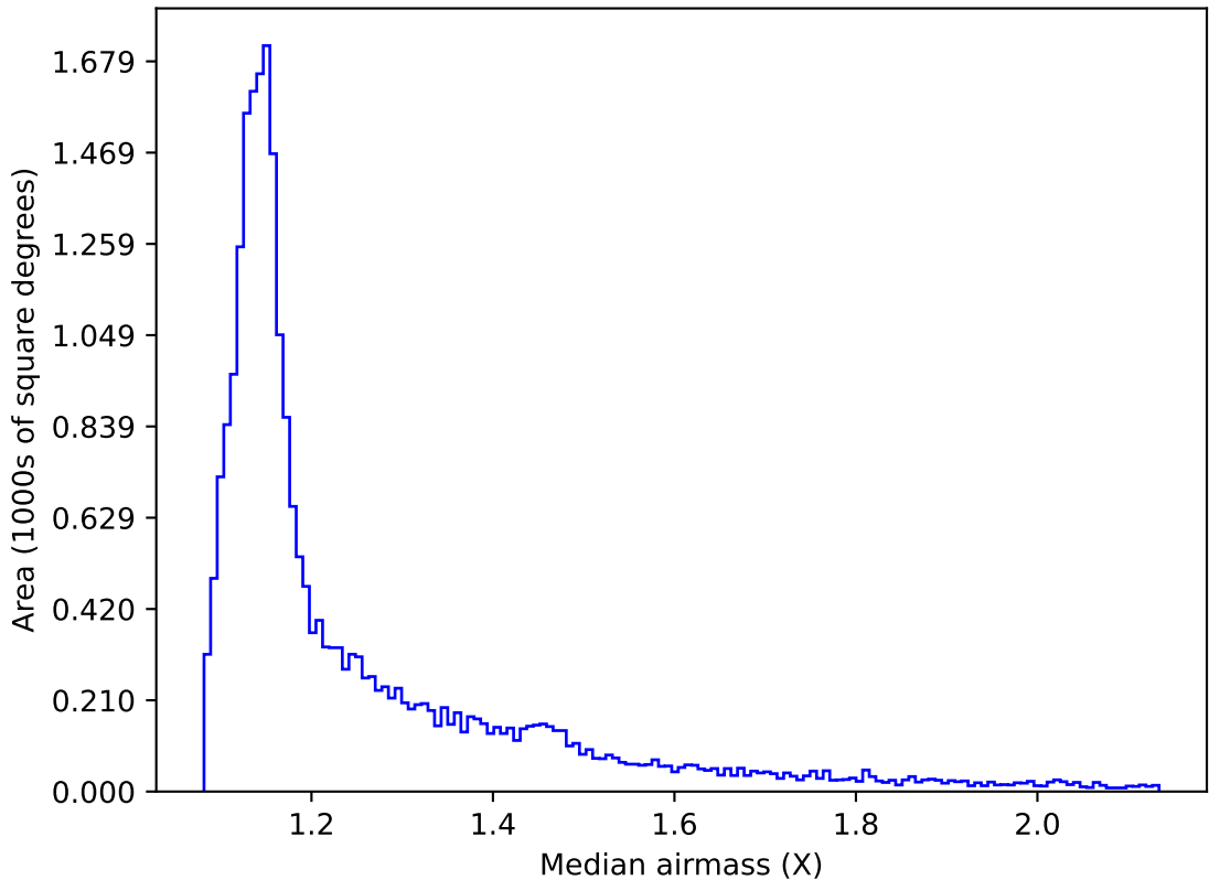
weather_cloudso8v3.4_10yrs All sky r band: Median airmass
