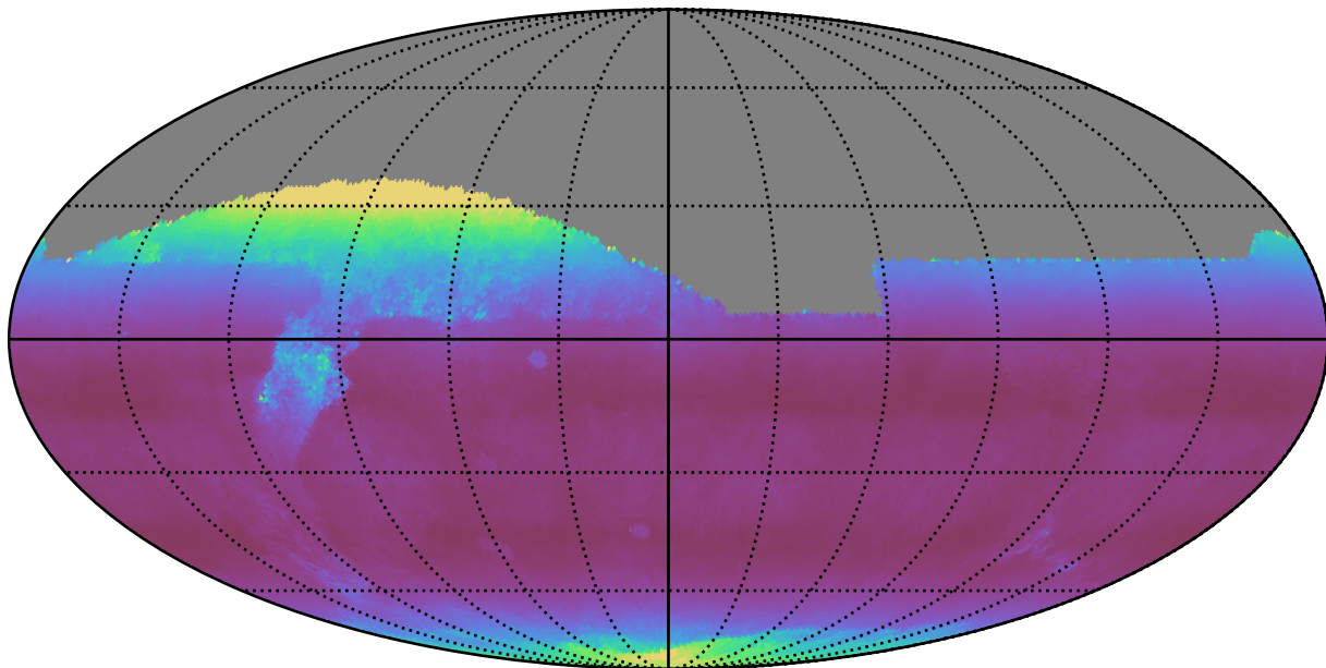
weather_cloudso8v3.4_10yrs All sky i band: Median airmass
