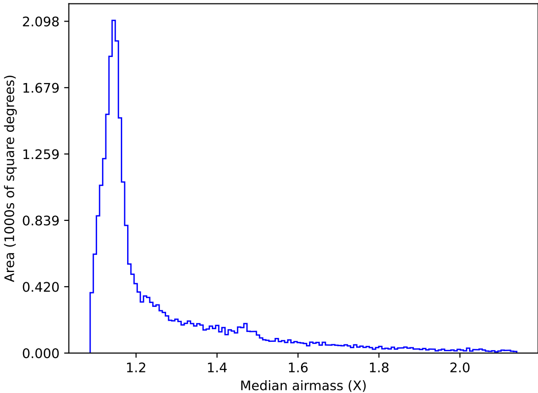
weather_cloudso8v3.4_10yrs All sky i band: Median airmass
