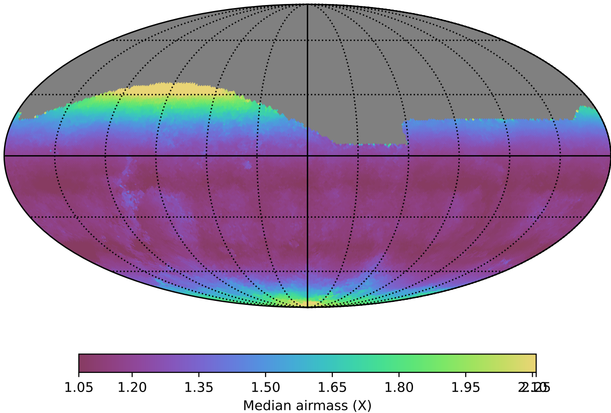
weather_cloudso8v3.4_10yrs All sky g band: Median airmass
