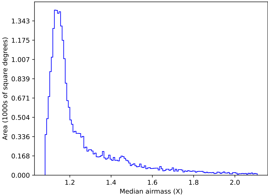
weather_cloudso8v3.4_10yrs All sky g band: Median airmass
