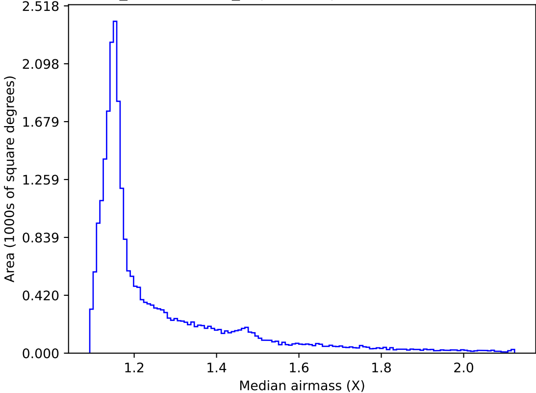
weather_cloudso8v3.4_10yrs All sky all bands: Median airmass
