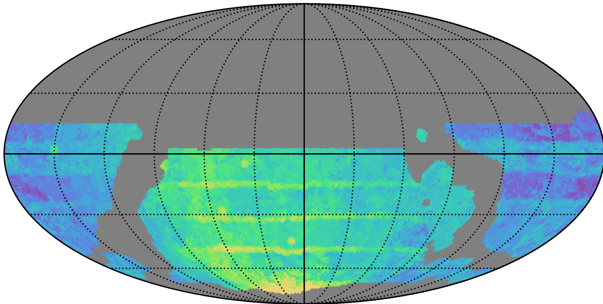
weather_cloudso8v3.4_10yrs WFD z band: Median Season Length
