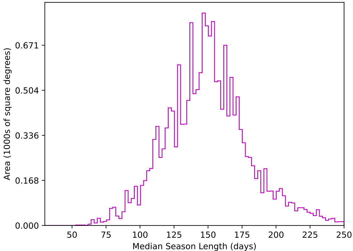
weather_cloudso8v3.4_10yrs WFD z band: Median Season Length
