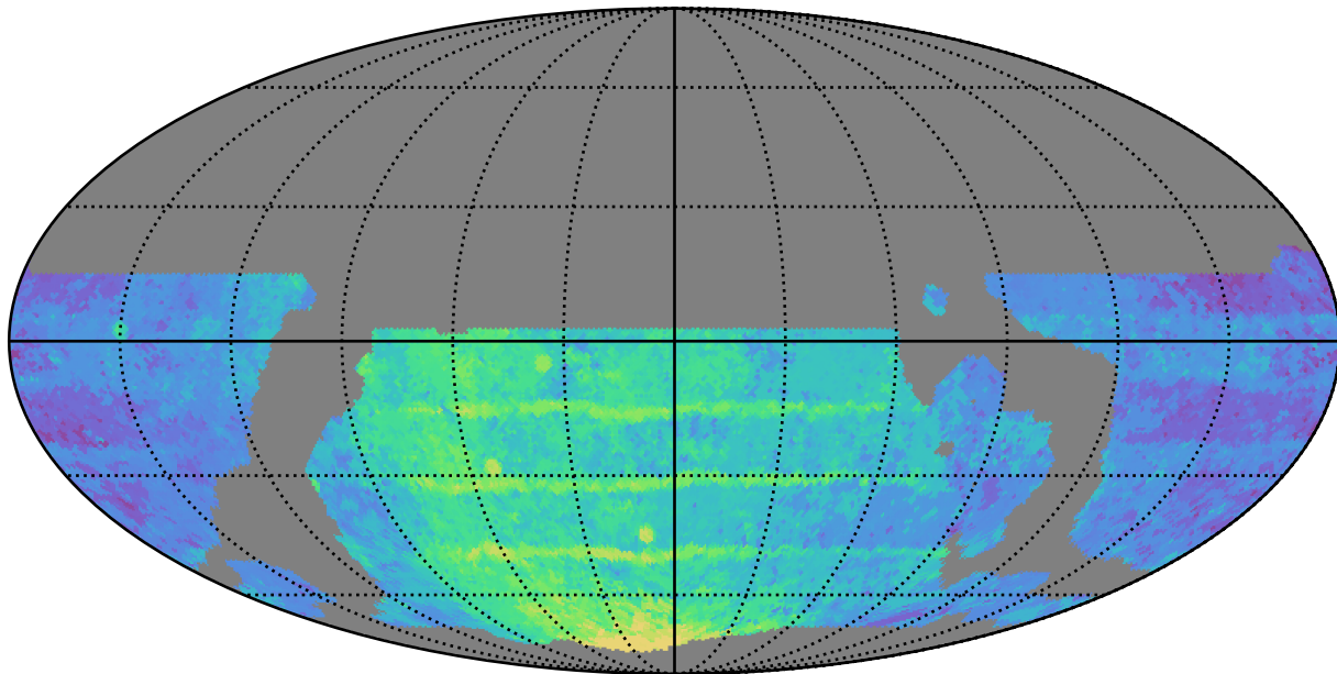
weather_cloudso8v3.4_10yrs WFD y band: Median Season Length
