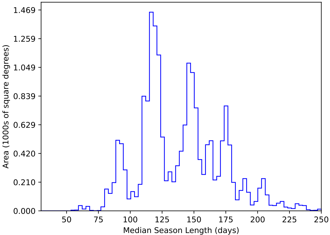
weather_cloudso8v3.4_10yrs WFD y band: Median Season Length
