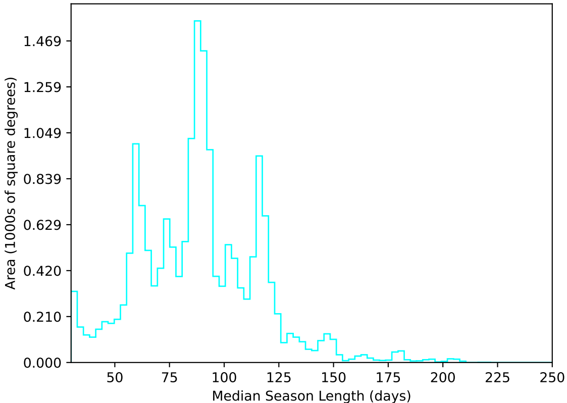
weather_cloudso8v3.4_10yrs WFD u band: Median Season Length
