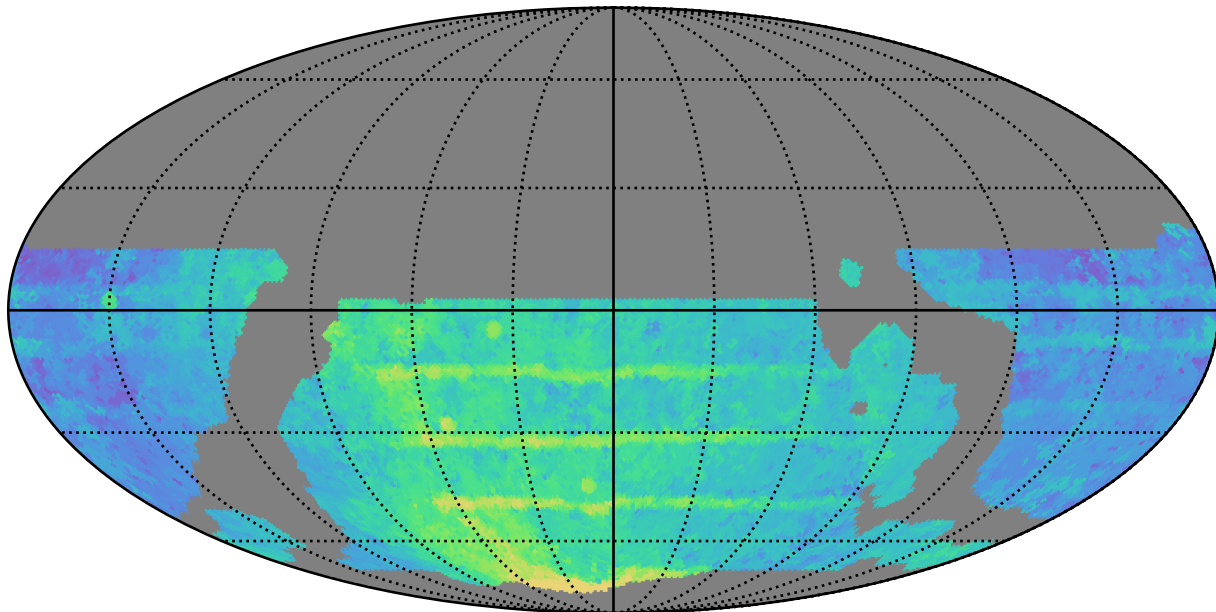
weather_cloudso8v3.4_10yrs WFD r band: Median Season Length
