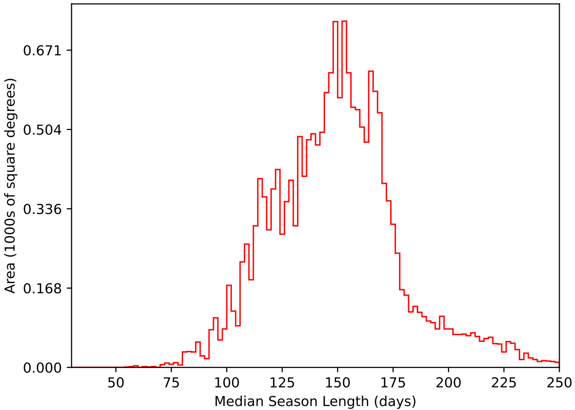
weather_cloudso8v3.4_10yrs WFD i band: Median Season Length
