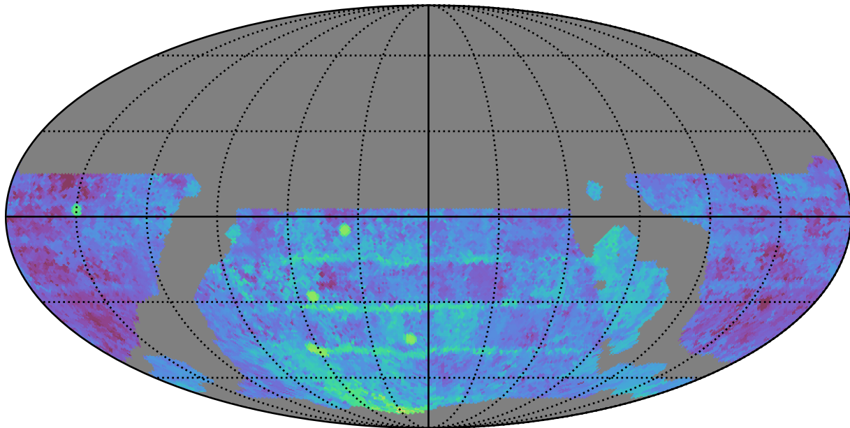
weather_cloudso8v3.4_10yrs WFD g band: Median Season Length
