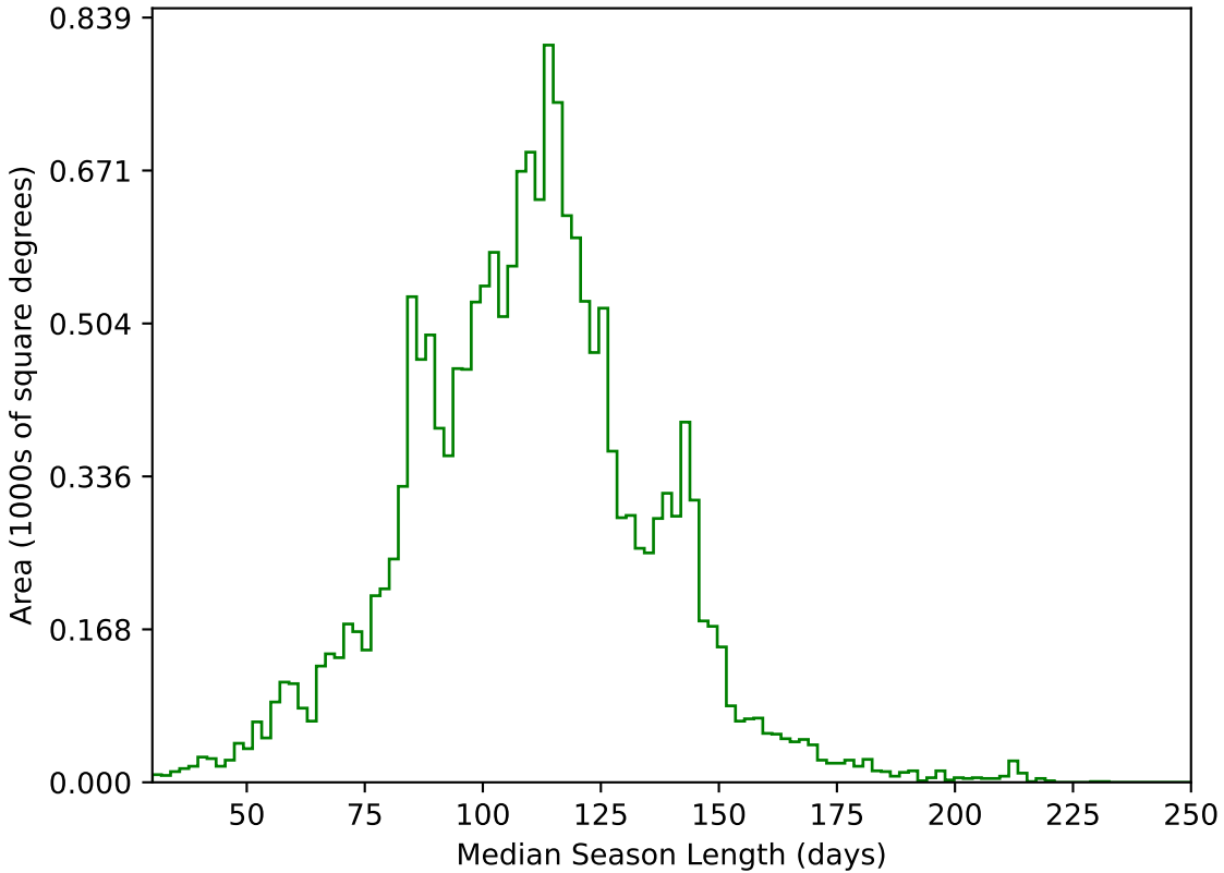
weather_cloudso8v3.4_10yrs WFD g band: Median Season Length
