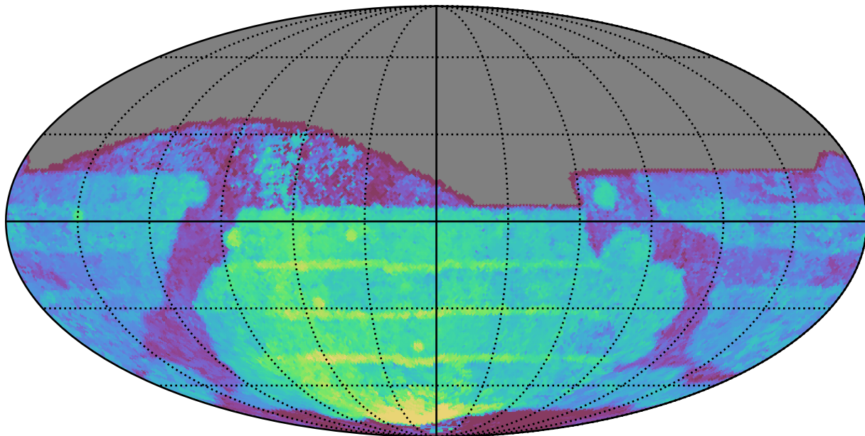
weather_cloudso8v3.4_10yrs All sky z band: Median Season Length
