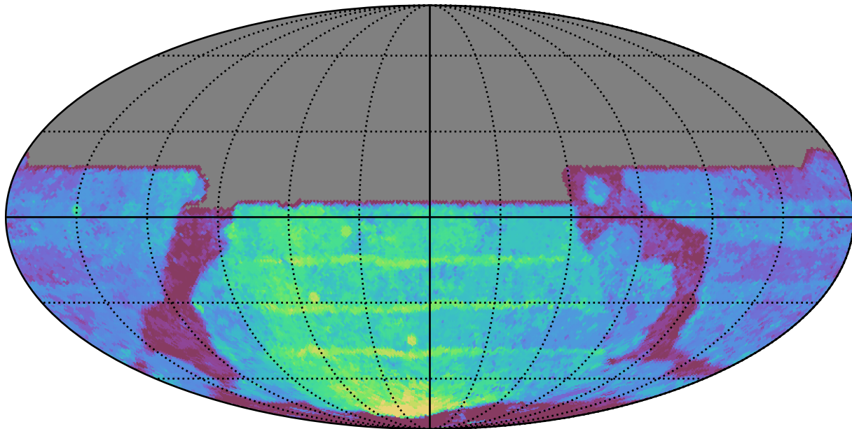
weather_cloudso8v3.4_10yrs All sky y band: Median Season Length
