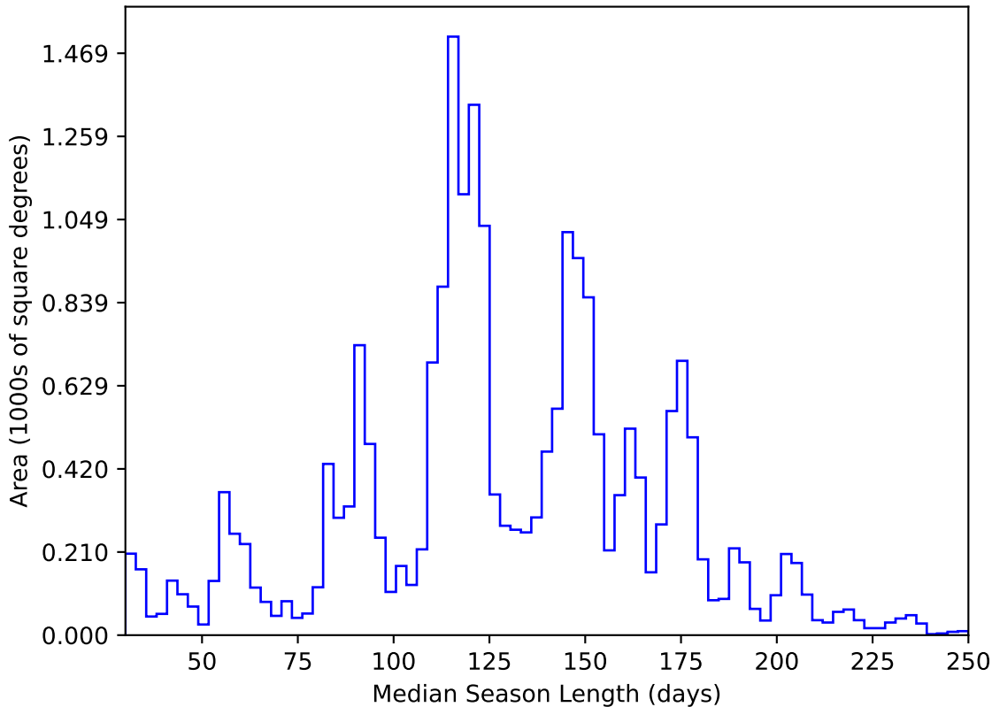
weather_cloudso8v3.4_10yrs All sky y band: Median Season Length
