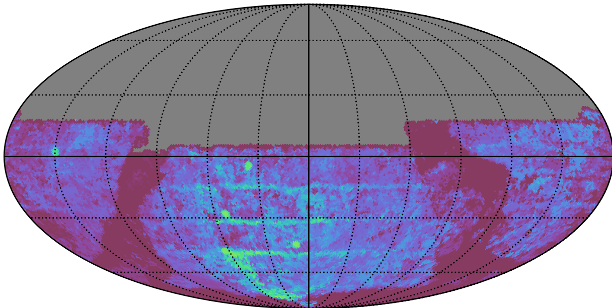
weather_cloudso8v3.4_10yrs All sky u band: Median Season Length
