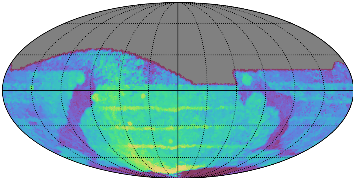
weather_cloudso8v3.4_10yrs All sky i band: Median Season Length
