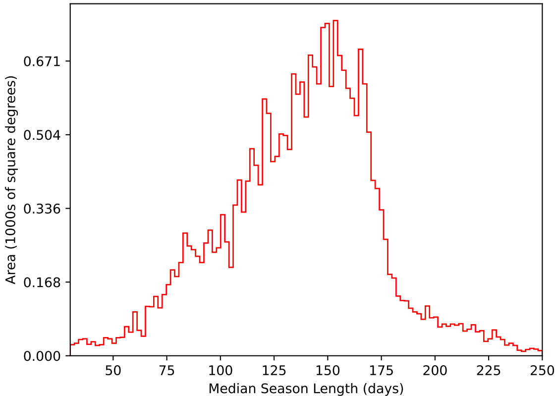
weather_cloudso8v3.4_10yrs All sky i band: Median Season Length
