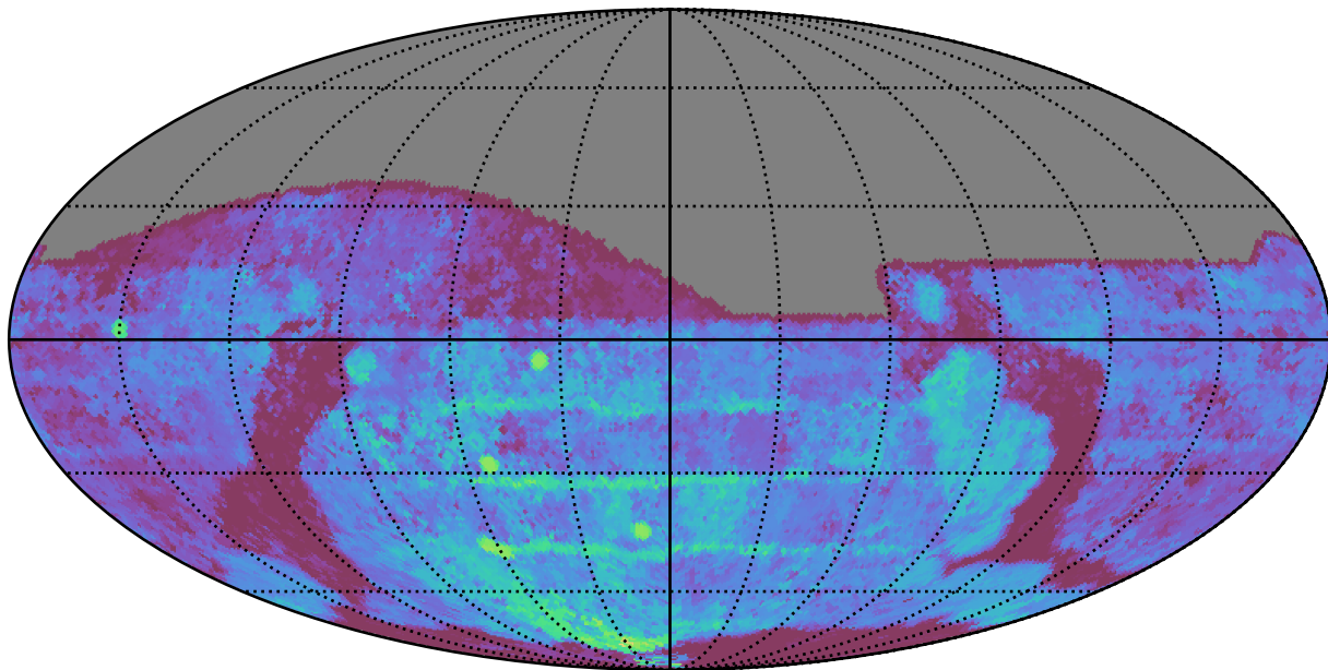
weather_cloudso8v3.4_10yrs All sky g band: Median Season Length
