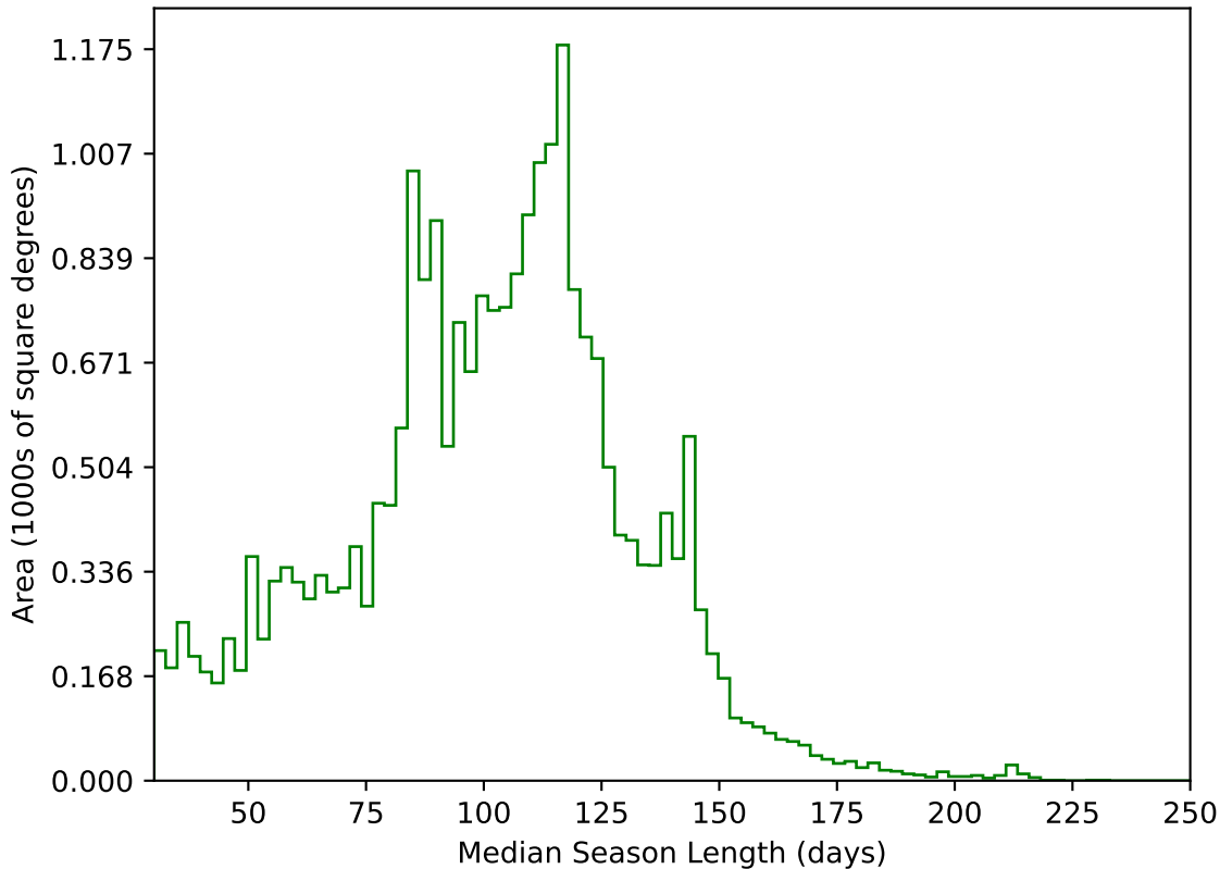
weather_cloudso8v3.4_10yrs All sky g band: Median Season Length
