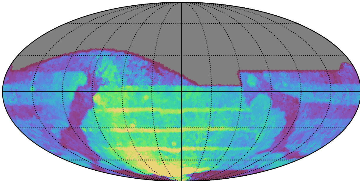
weather_cloudso8v3.4_10yrs All sky all bands: Median Season Length
