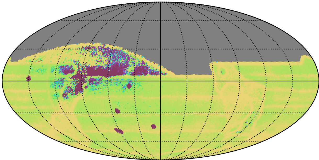
weather_cloudso8v3.4_10yrs All sky: Median Intra-Night Gap
