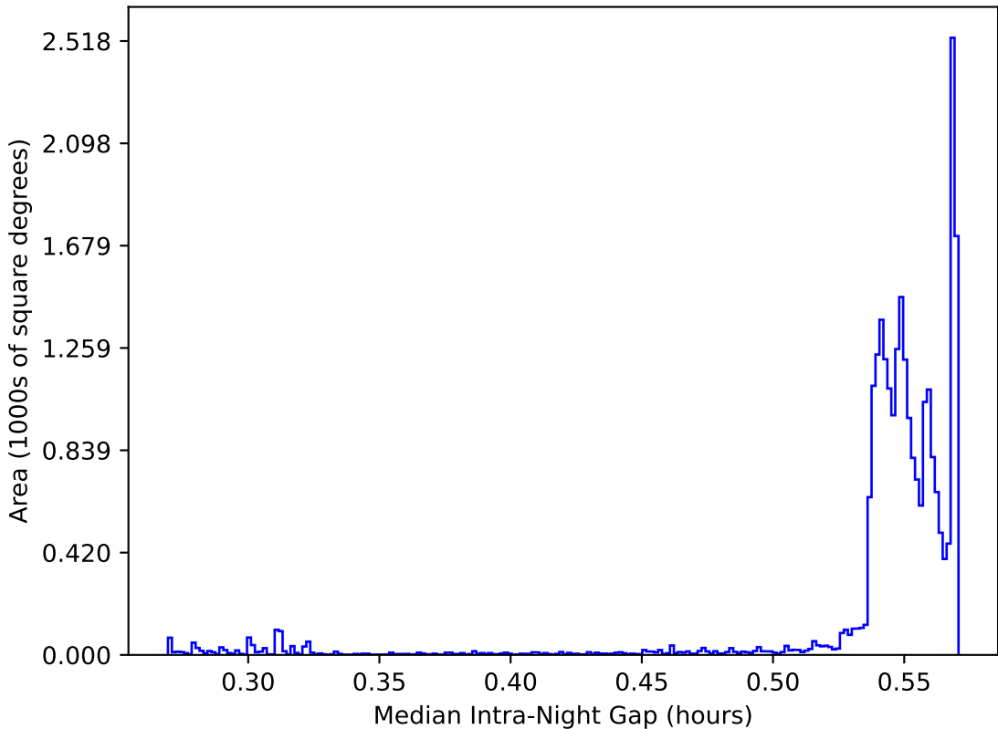
weather_cloudso8v3.4_10yrs All sky: Median Intra-Night Gap
