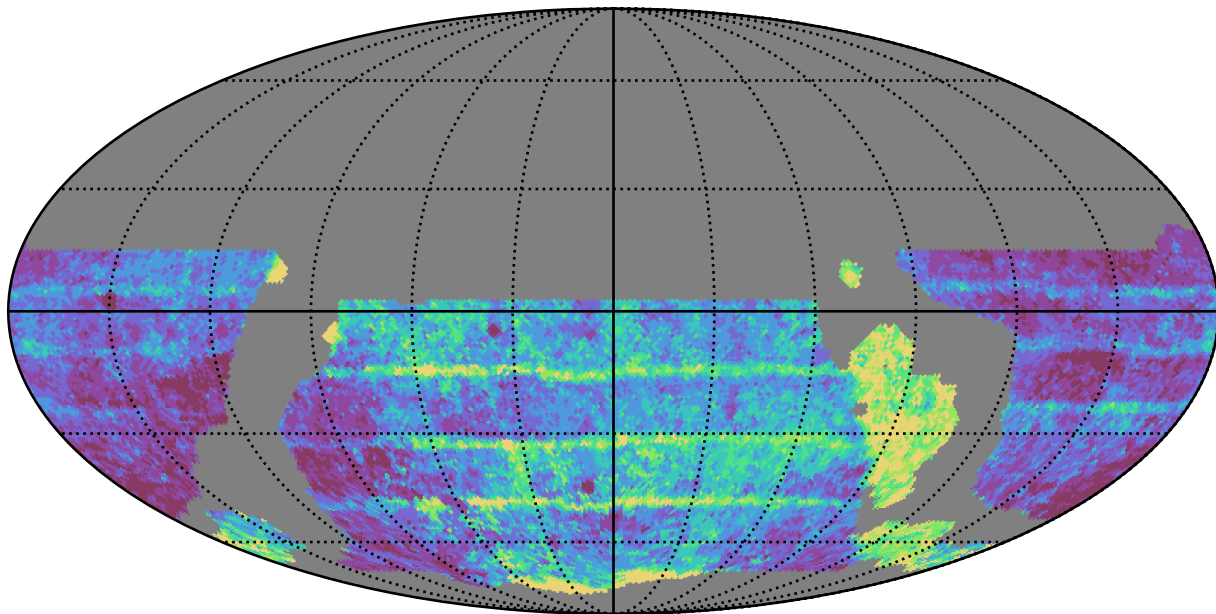
weather_cloudso8v3.4_10yrs WFD z band: Median Inter-Night Gap
