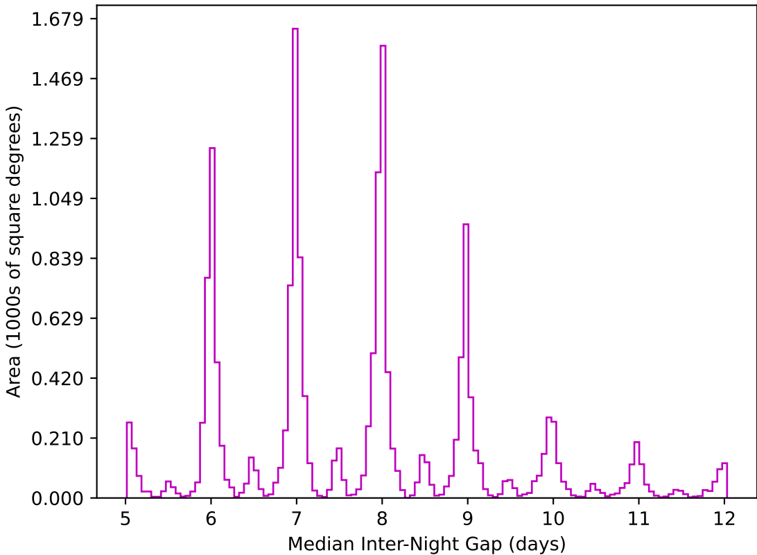
weather_cloudso8v3.4_10yrs WFD z band: Median Inter-Night Gap
