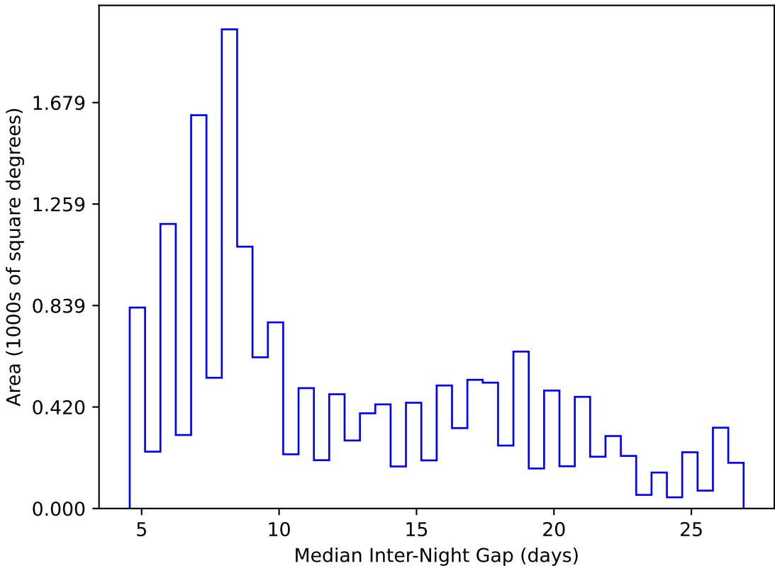
weather_cloudso8v3.4_10yrs WFD y band: Median Inter-Night Gap
