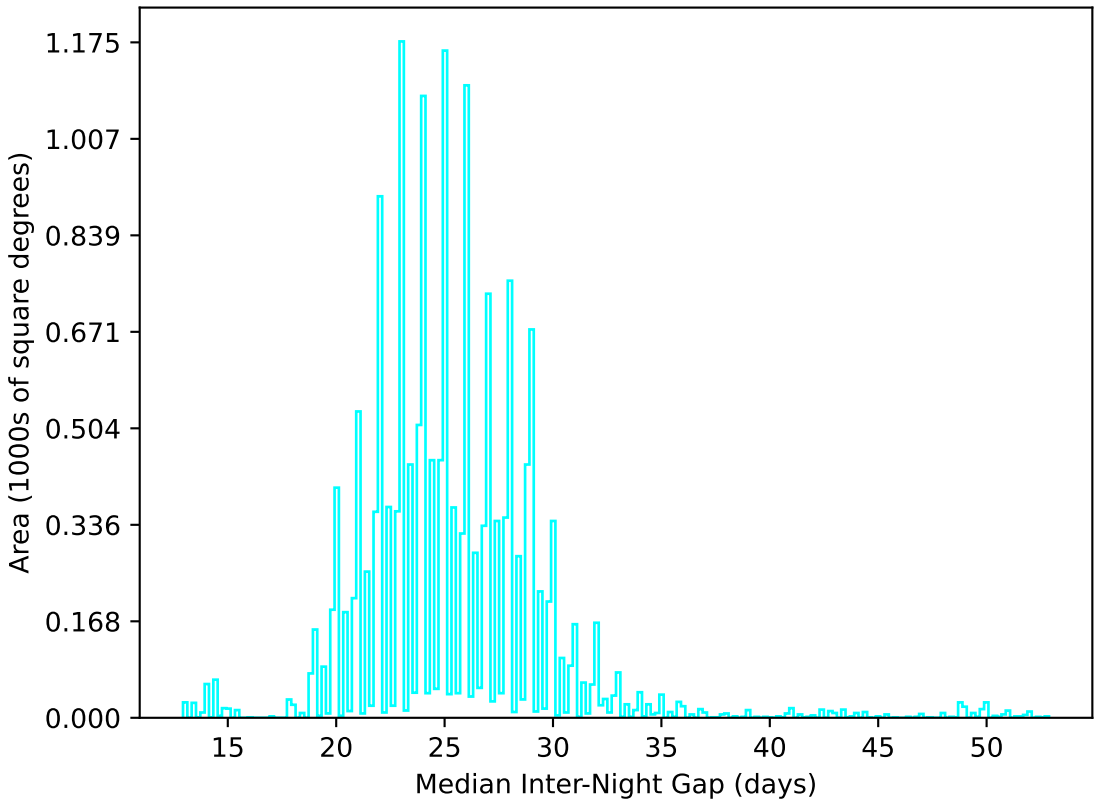
weather_cloudso8v3.4_10yrs WFD u band: Median Inter-Night Gap
