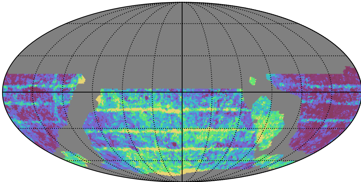
weather_cloudso8v3.4_10yrs WFD i band: Median Inter-Night Gap
