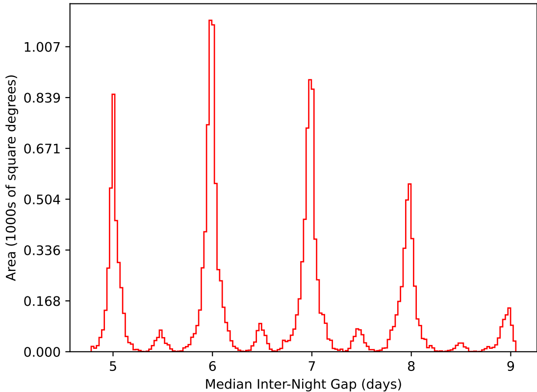
weather_cloudso8v3.4_10yrs WFD i band: Median Inter-Night Gap
