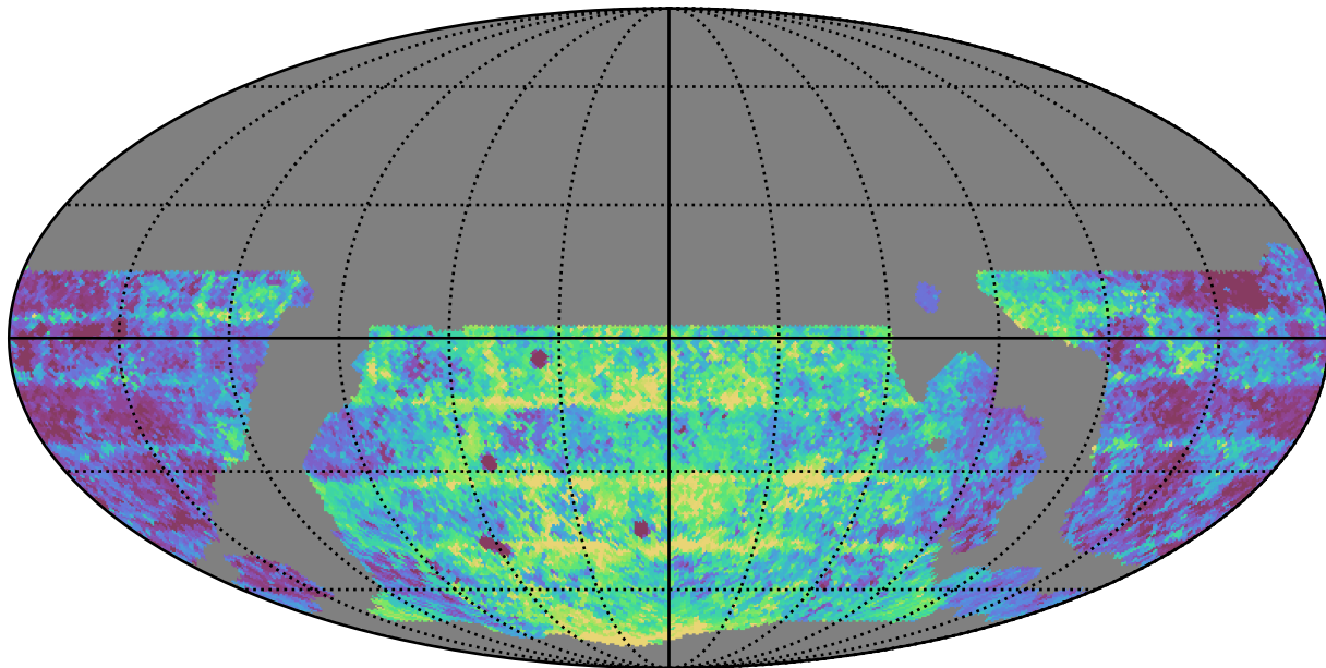
weather_cloudso8v3.4_10yrs WFD g band: Median Inter-Night Gap
