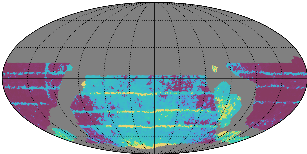
weather_cloudso8v3.4_10yrs WFD all bands: Median Inter-Night Gap
