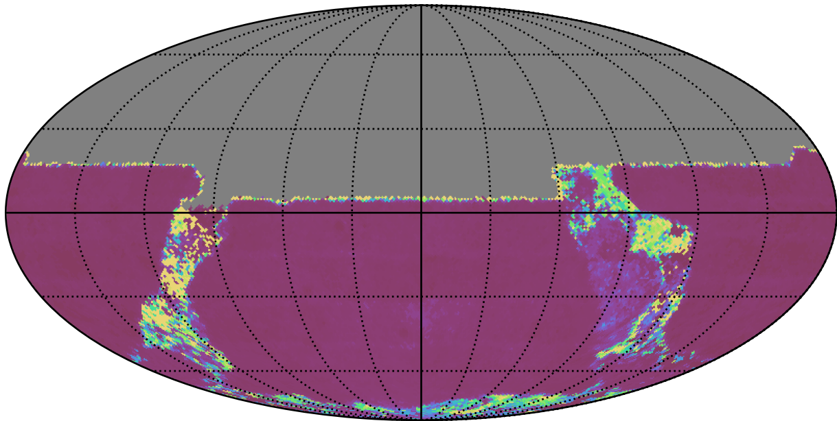
weather_cloudso8v3.4_10yrs All sky u band: Median Inter-Night Gap
