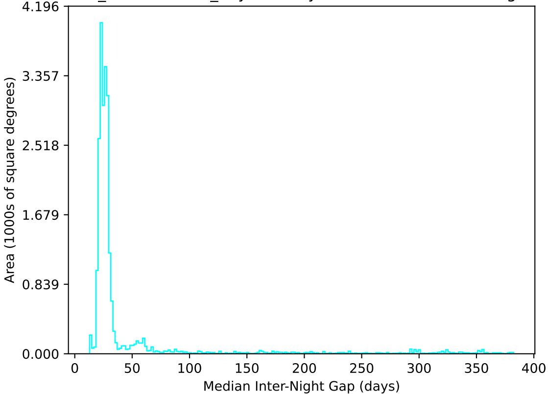
weather_cloudso8v3.4_10yrs All sky u band: Median Inter-Night Gap
