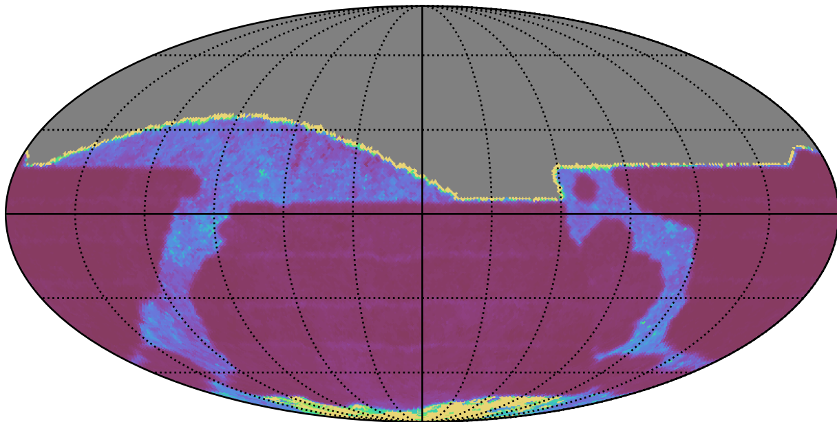
weather_cloudso8v3.4_10yrs All sky r band: Median Inter-Night Gap
