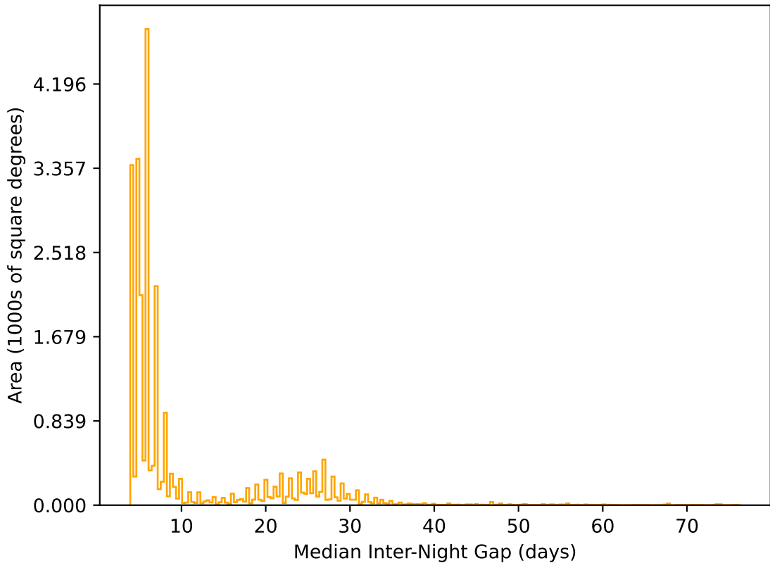
weather_cloudso8v3.4_10yrs All sky r band: Median Inter-Night Gap
