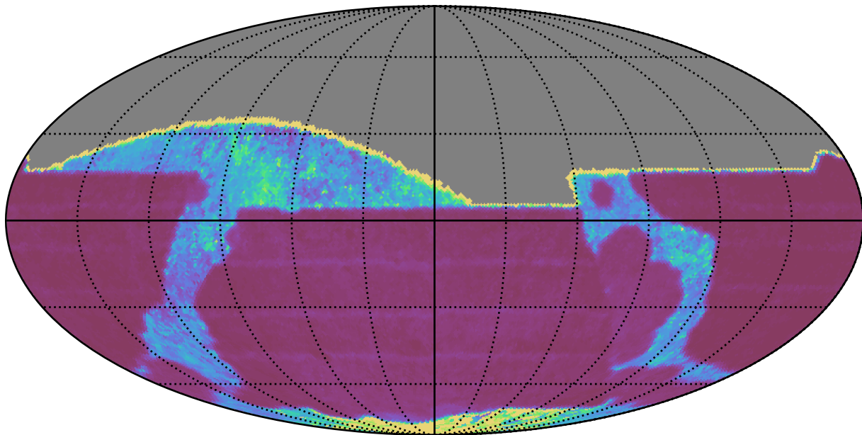
weather_cloudso8v3.4_10yrs All sky i band: Median Inter-Night Gap
