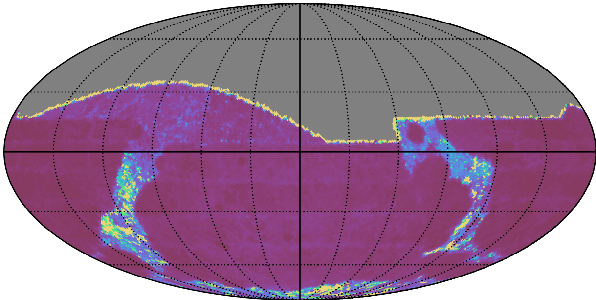
weather_cloudso8v3.4_10yrs All sky g band: Median Inter-Night Gap
