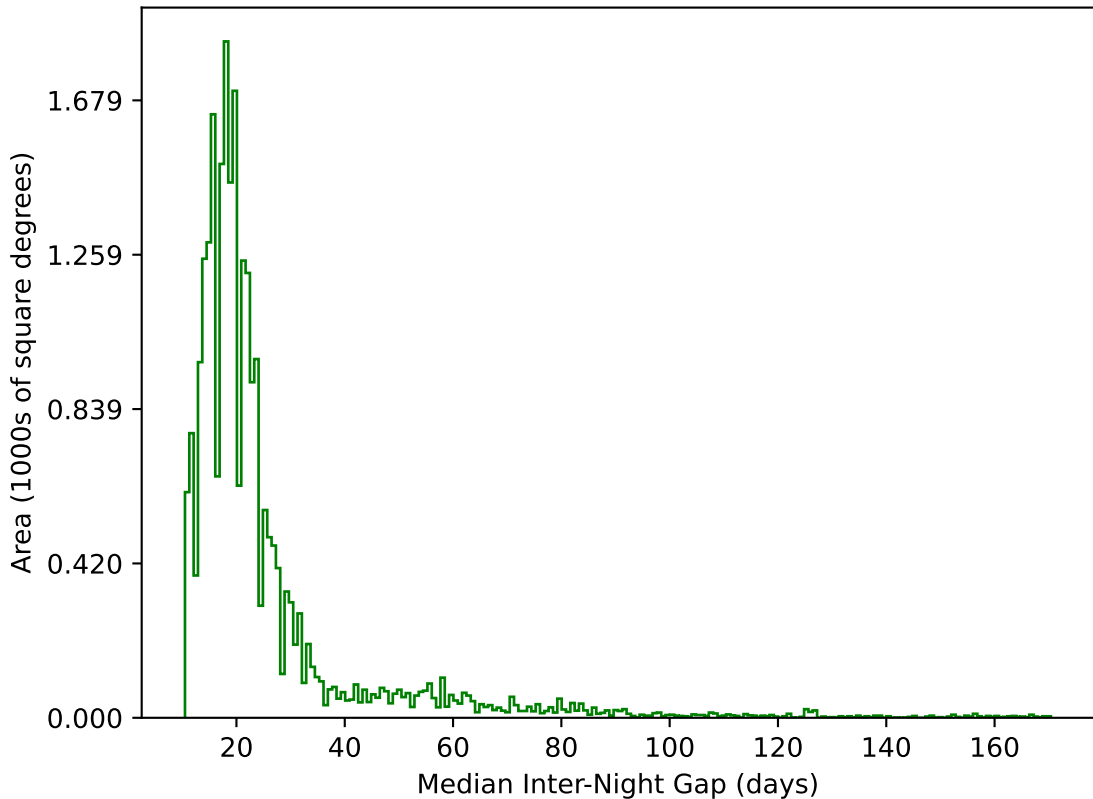
weather_cloudso8v3.4_10yrs All sky g band: Median Inter-Night Gap
