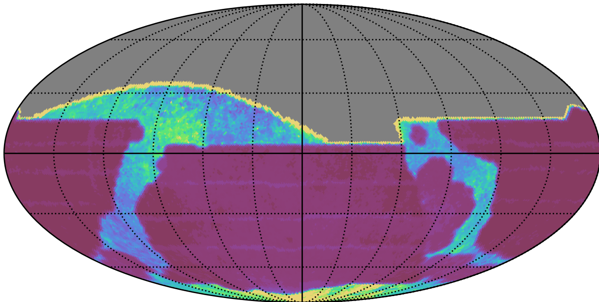
weather_cloudso8v3.4_10yrs All sky all bands: Median Inter-Night Gap
